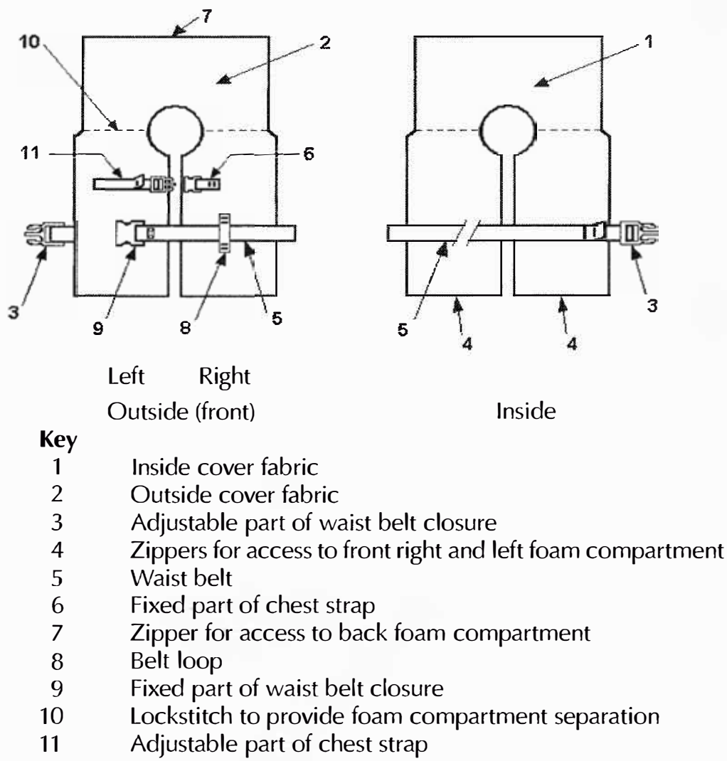
Figure B.1 – General arrangement, right side out (outside and inside)
