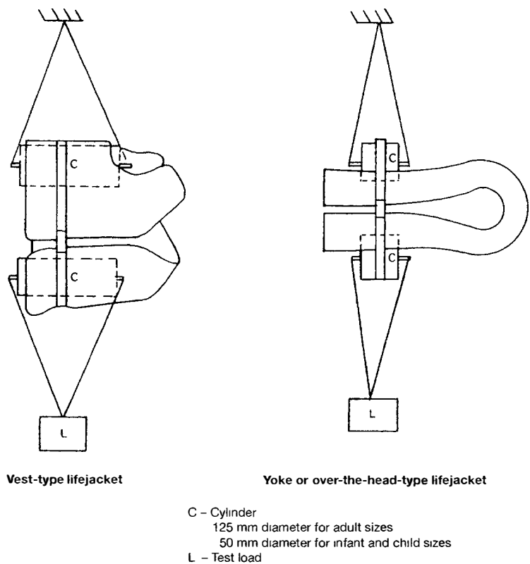
Figure 1 – Body strength test arrangement for lifejackets
