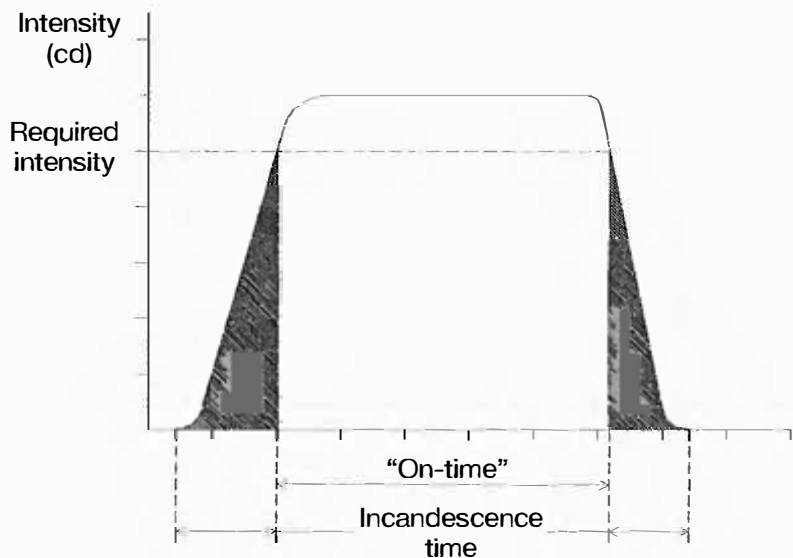
Figure 10.4.1 – “On-time” measurement diagram
