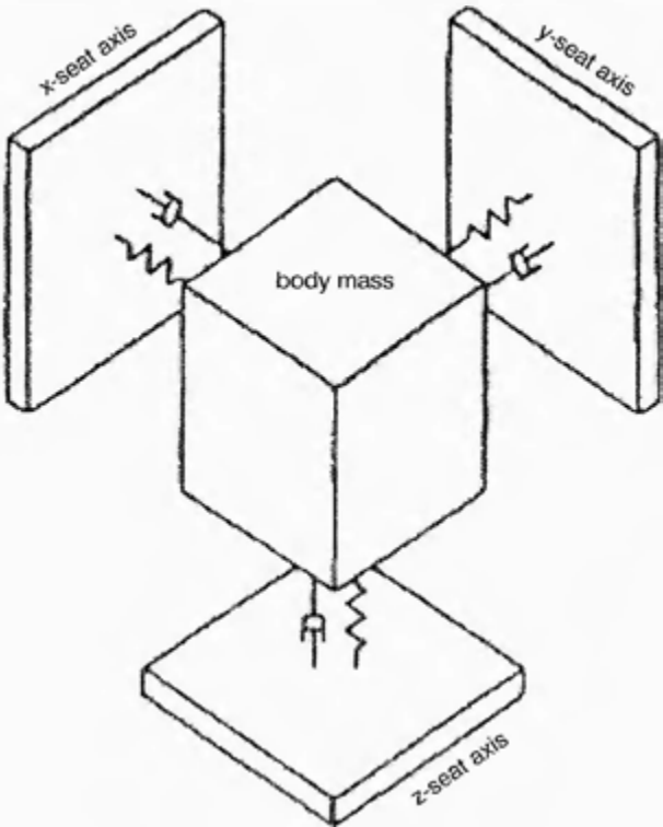
Figure 3 – Independent single-degree-of-freedom representation of human body
