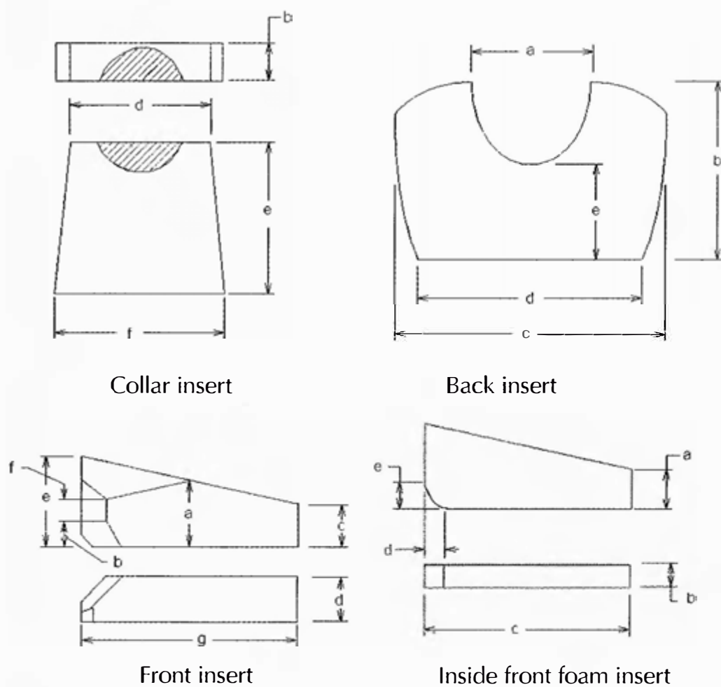
Figure 1 – Adult RTD foam insert nomenclature
