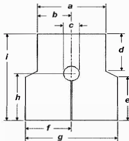
Figure C.4 – Cover cut pattern (outside and inside covers)
