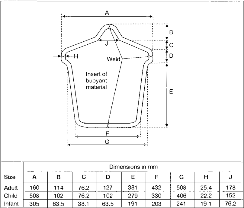
Figure 2 – Test form for shoulder lift test for lifejackets
