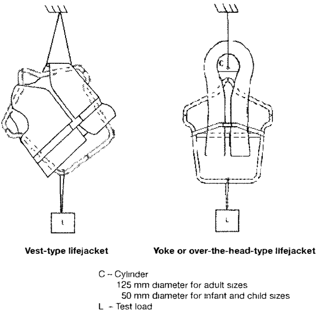
Figure 3 – Shoulder lift test arrangement for lifejackets
