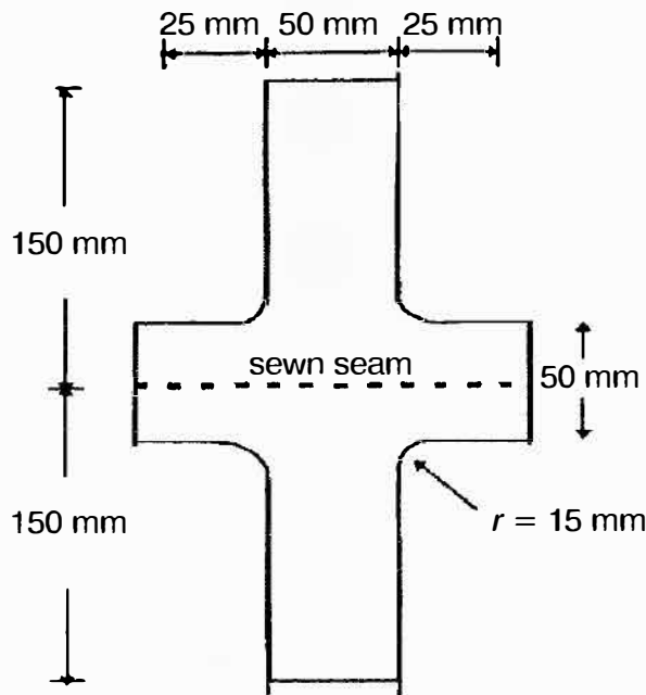
Figure 1 – Sample specification for sewn canopy seams
