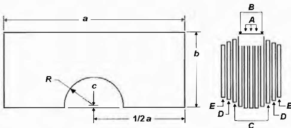
Figure B.3 – Back foam insert
