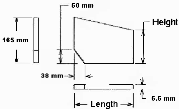
Figure 2 – Adult RTD “make-up” foam insert sizes
